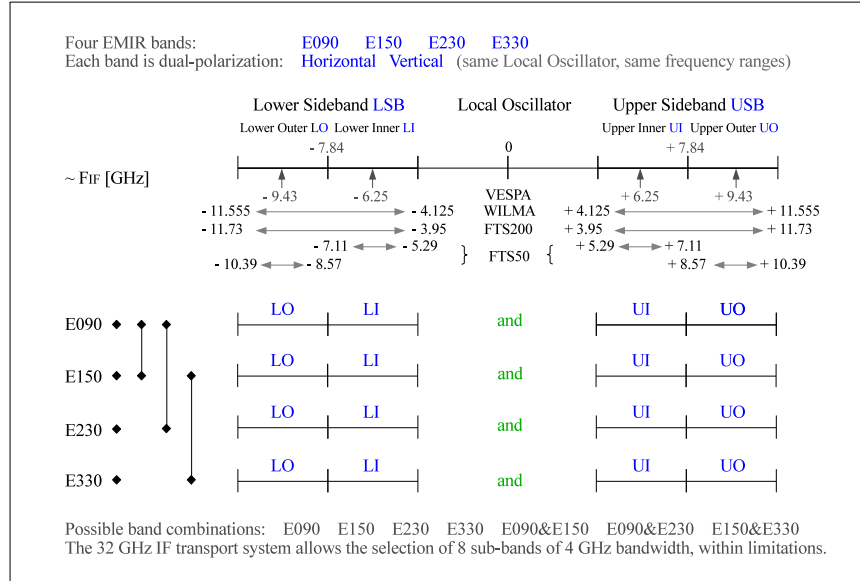
Figure 2: Visual overview of EMIR bands since the E 150 mixer upgrade conducted in autumn 2013. Eight sub-bands can be transported to backends for a total of 32 GHz instantaneous bandwidth. Frequencies shown above the frequency scale indicate the central frequencies of the (sub-)bands. Frequencies at the sideband edges give the frequency coverage of the backends.
