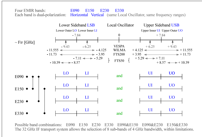
Figure 2: Visual overview of EMIR bands after the E 150 mixer upgrade planned for autumn 2013. Eight sub-bands can be transported to backends for a total of 32 GHz instantaneous bandwidth. Frequencies shown above the frequency scale indicate the central frequencies of the (sub-)bands. Frequencies at the sideband edges give the frequency coverage of the backends.
