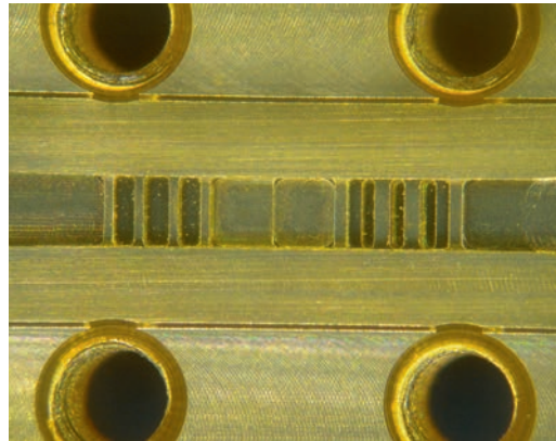
Close view on the 135-184 GHz band-pass filter for the NOEMA Band 2 local oscillator. It consists of the combination of one high-pass filter given by the waveguide cutoff and a low-pass filter whose rejection frequency is fixed by the 0.22 \pm 0.01 mm large and 0.41 \pm 0.01 mm deep slots.
