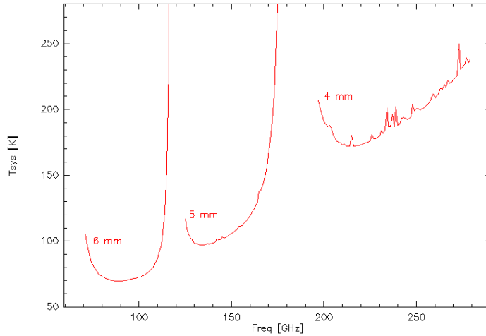
Figure 1: Summer 2018 semester T_{\text{sys}} for 20 degrees declination source (maximum elevation 65 deg). The numbers indicate the precipitable water vapour (PWV) values assumed in the computation.
